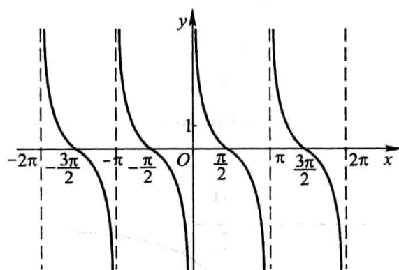
y = \cot x
