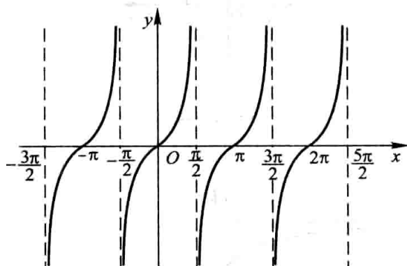
y = \tan x
